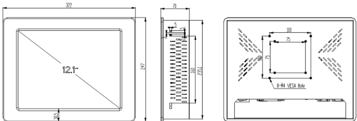
CUT OUT DIMENSION(309.5x237mm) UNIT:mm
